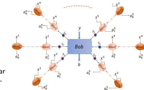
Device-independent nonlocal correlation in Star network
