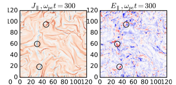
Plasma Turbulence
