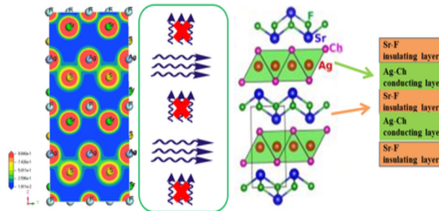
Charge flow in a layered structure of SrAgChF
